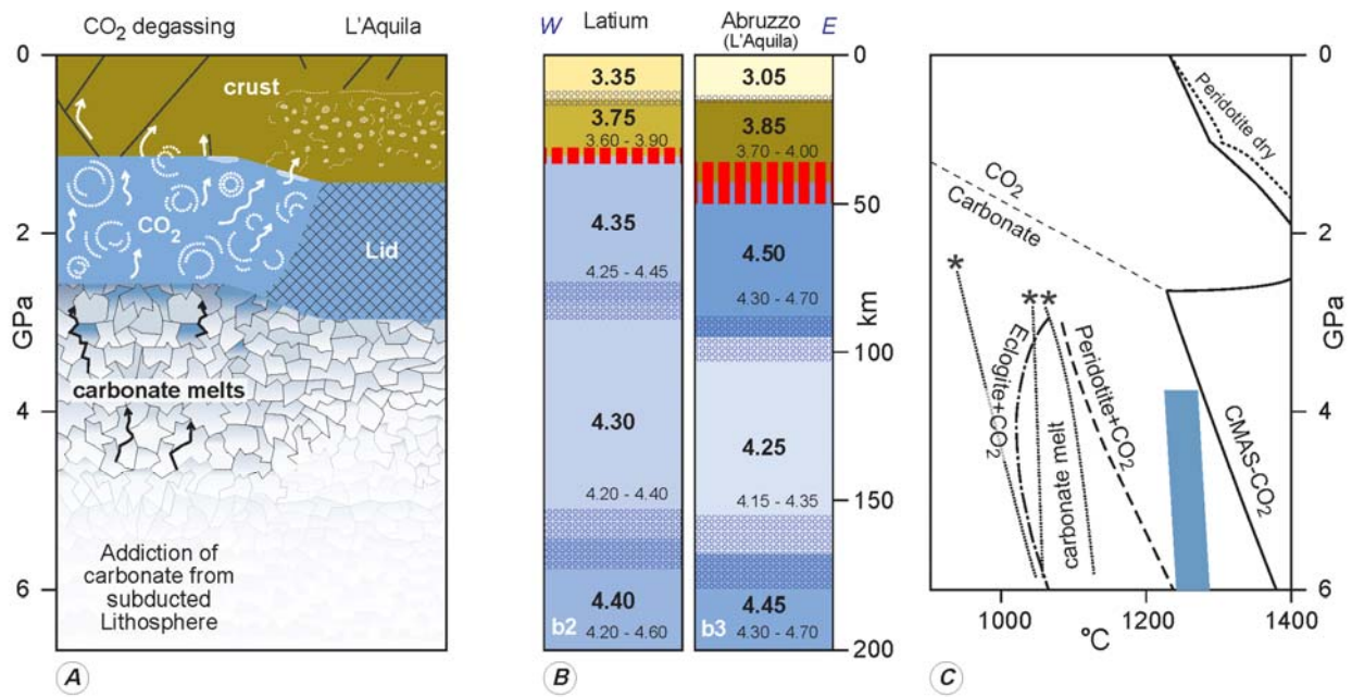
Figure 2. Present-day architecture of mantle-CO 2 degassing beneath L'Aquila (Central Italy).
