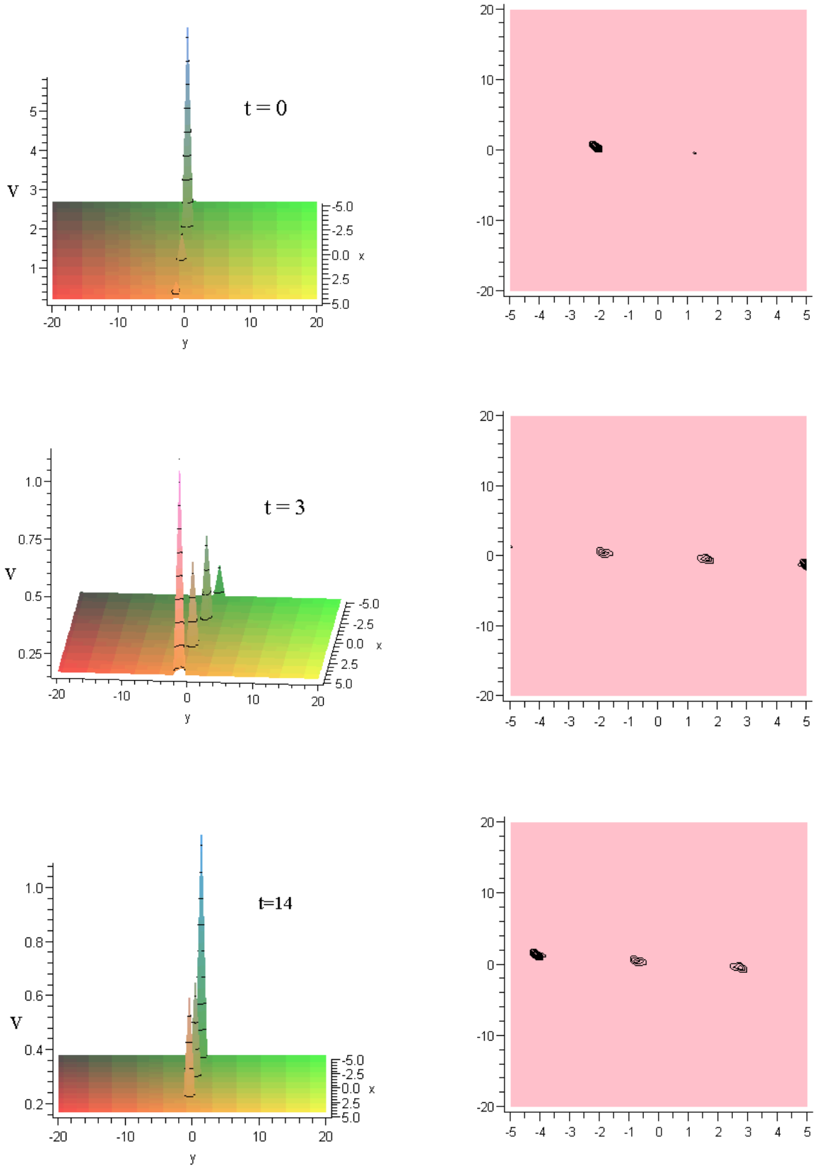
Figure 2: Propagating multidromion-like solutions v(x,y,t) for various instants of time.
