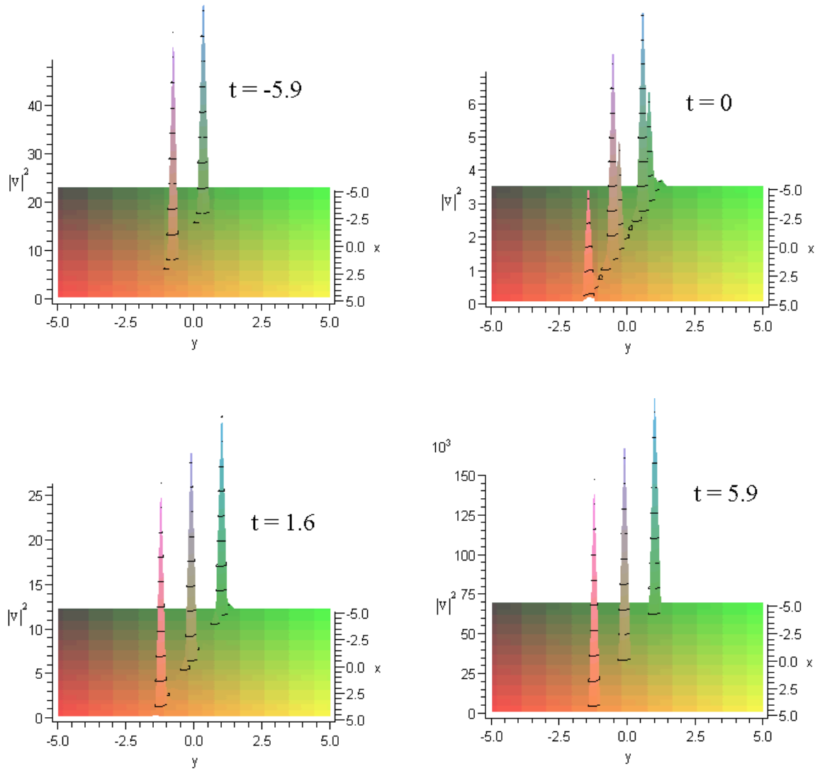
Figure 3: Snap-shots of the envelop of the multidromion-like profile at various instants of time.
