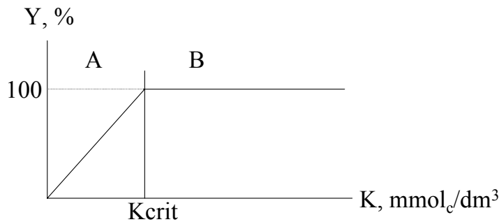
Figure 9. The relative grain yield ( Y , %) as function of soil potassium content ( K , \text{mmol}_c \cdot \text{dm}^3 ): (A) deficient soil fertility, (B) sufficient soil fertility, and the critical soil potassium content ( K_{\text{crit}} , \text{mmol}_c \cdot \text{dm}^3 ).
