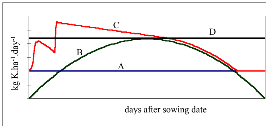
Figure 8. The potassium availability in the soil expressed in terms of offer rate: (A) deficient soil fertility, (C) deficient soil fertility with two fertilizations, (D) sufficient soil fertility, and (B) the crop potassium requirement rate ( \text{kg K}\cdot\text{ha}^{-1}\cdot\text{day}^{-1} ).
