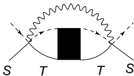
FIG. 4: Phonon and parquet corrections to the vertex \gamma_B . Solid and dashed lines denote spin-fermion and conduction electron propagators, all parquet series are incorporated in the insertion shown by the square box. The multiphonon propagator is shown by the wavy line.
