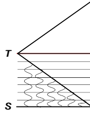
FIG. 2: n -phonon processes connect singlet with spin 1 projection of triplet ( n\hbar\Omega < \Delta ).
