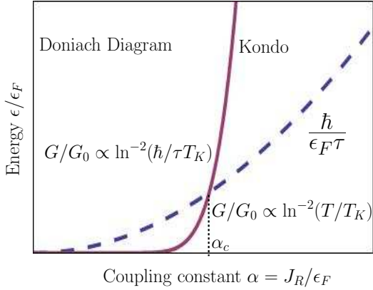
FIG. 5: Phase diagram illustrating the competition between Kondo temperature and relaxation damping. Solid line stands for characteristic Kondo energy. Dashed line corresponds to the damping parameter. The phonon-assisted Kondo tunneling is effective for \alpha > \alpha_c , where \alpha_c \sim 10^{-2} for TMOC coupled with metallic leads. G/G_0 is enhancement factor for ZBA in tunnel conductance.
