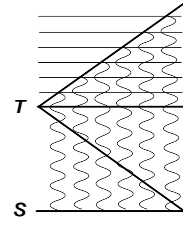
FIG. 3: (n + m) -phonon processes connect singlet with spin \bar{1} projection of triplet ( (n + 1)\hbar\Omega > \Delta ).
