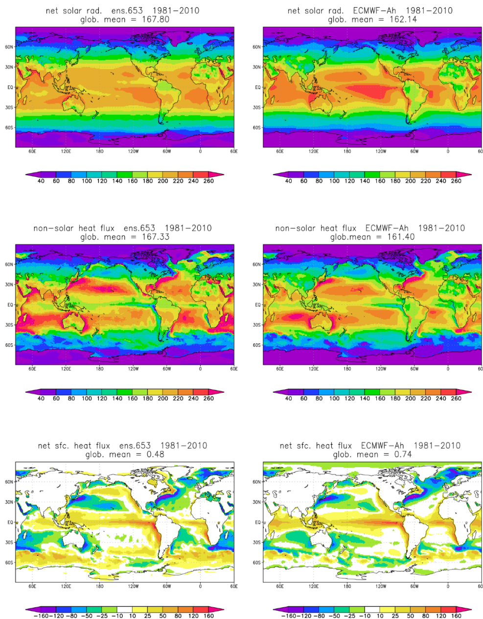
365 Figure 4: Left column: annual-mean climatology (for 1981-2010) of solar (top), non-solar (centre), and net surface heat fluxes (bottom), in W/m 2 , simulated by the SPEEDY ensemble with prescribed SST (ens.653). Solar and net fluxes are downward, non-solar flux is upward. Right column: as in left column, but from an ensemble of 65-yr simulations with prescribed SST run at ECMWF (ECMWF-Ah; Roberts et al. 2018).
