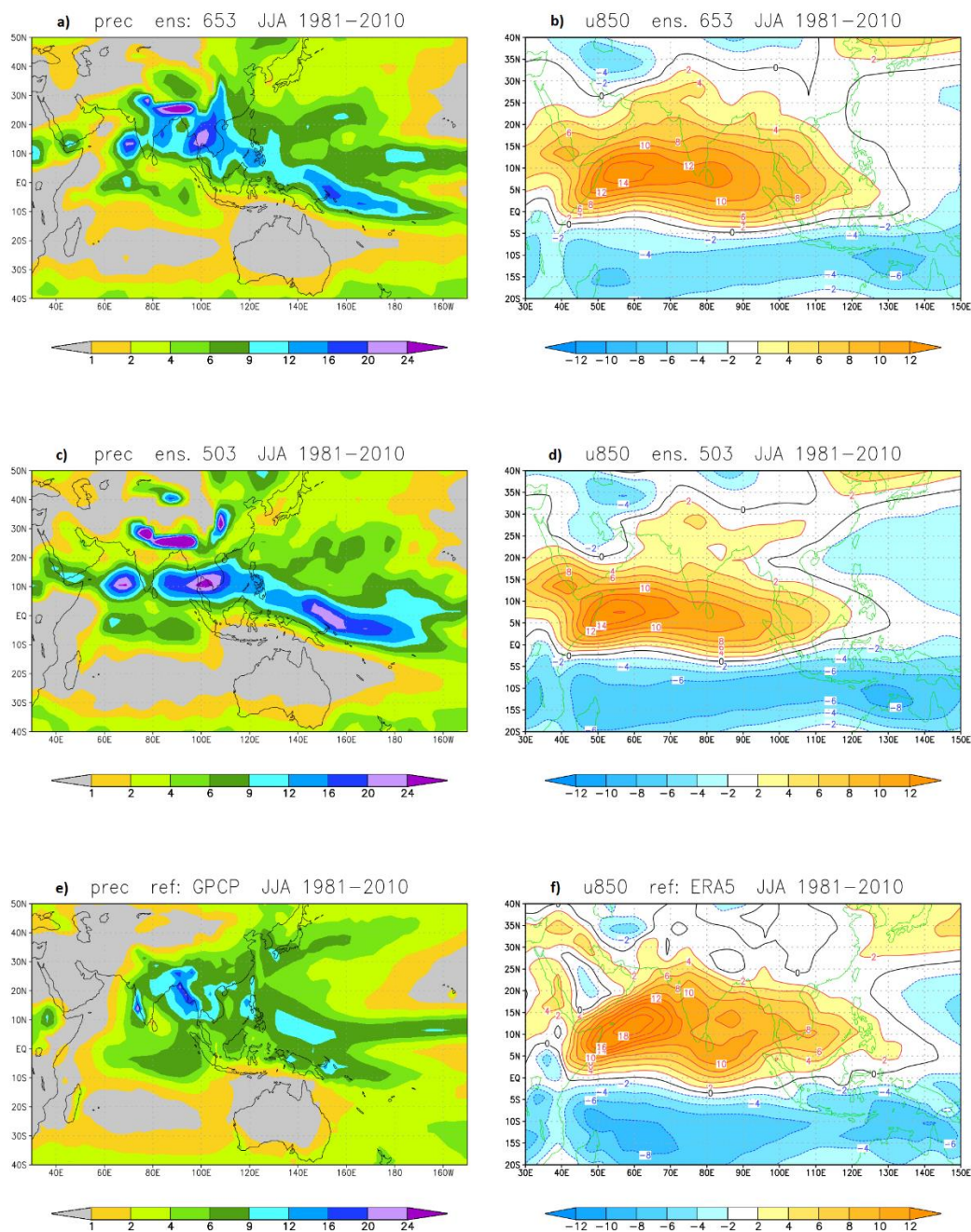
Figure 7: Asian monsoon rainfall (left, in mm/day) and 850-hPa zonal wind (right, in m/s) in SPEEDY ensembles with prescribed SST, for JJA 1981–2010. a) and b): ensemble with v.42 (ens.653). c) and d): ensemble with v.42 dynamics but v.41 parametrizations (ens.503). e): rainfall climatology from GPCPv2.3 (Adler et al. 2003). f): zonal wind climatology from ERA5.
