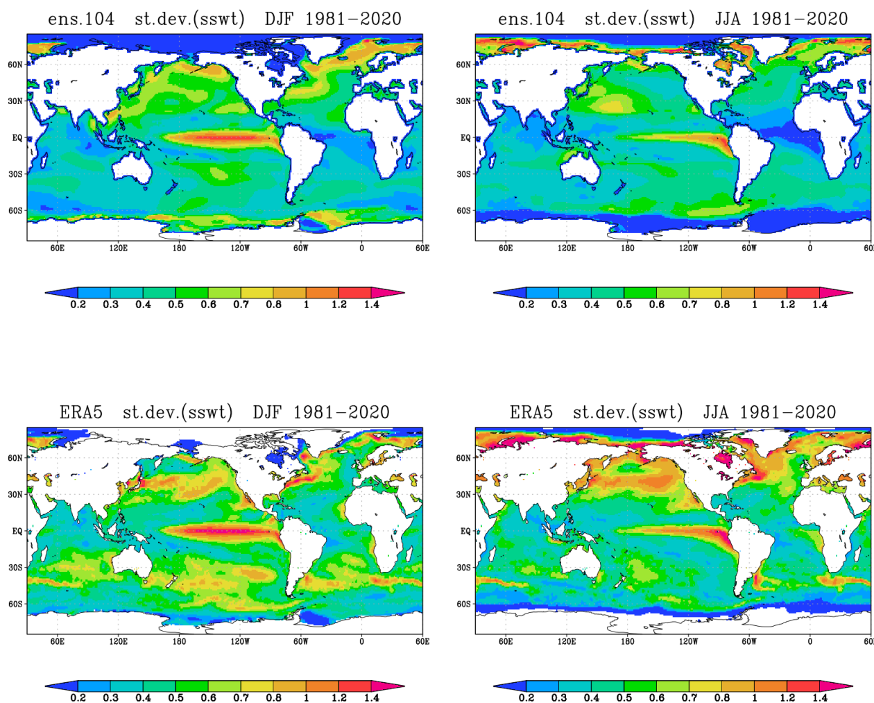
Figure 11: Interannual variability of SSWT in DJF 1981-2020 (left) and JJA 1981-2020 (right), from the SPEEDY-TOM3 ensemble (ens.104, top) and ERA5 (bottom). Data are standard deviations of seasonal means, in °K
