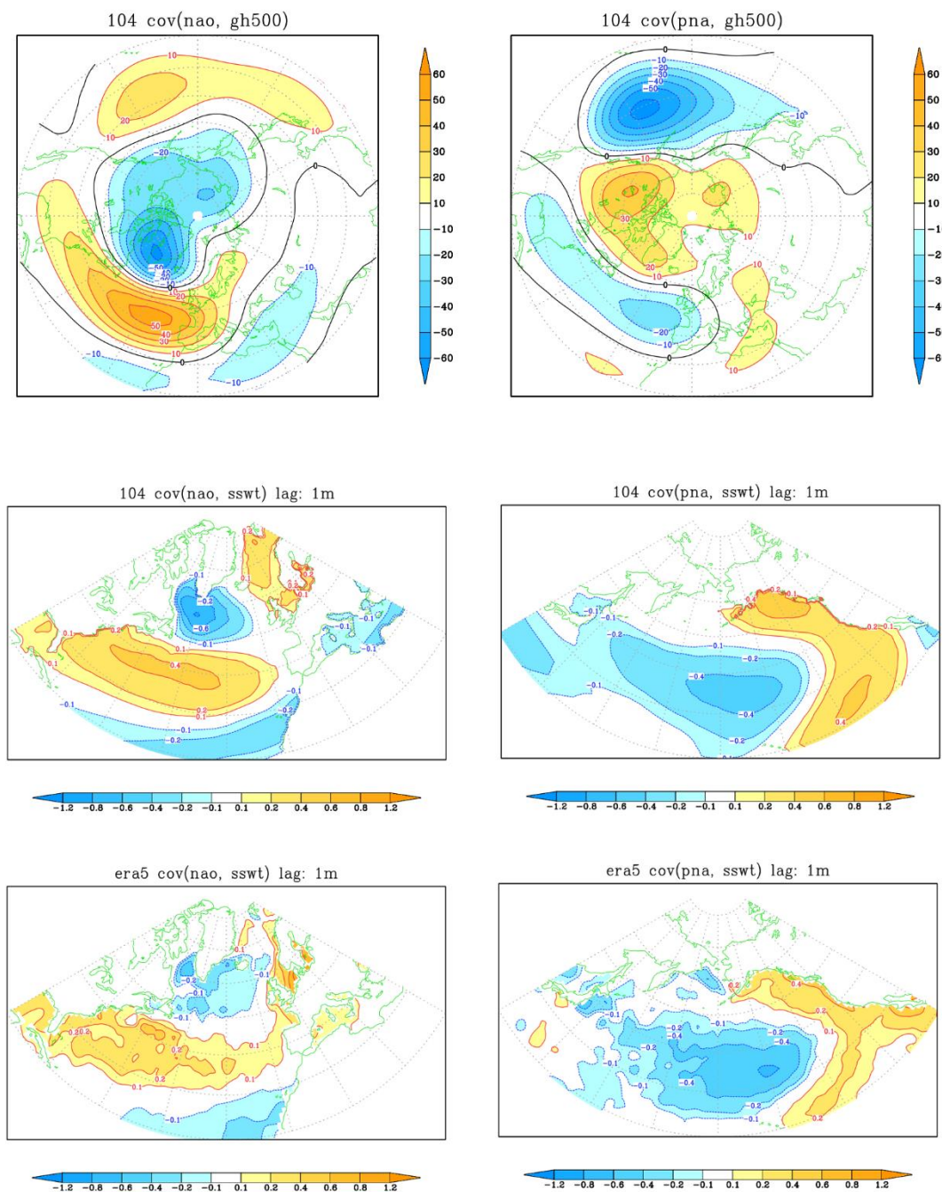
Figure 12: Covariances with the NAO (left) and PNA (right) indices in JF 1981-2020, as defined in Sect. 3.2. Top: covariance with 500-hPa height (in m) in the coupled ensemble (ens.104). Centre: 1-month-lag covariance with February-March SSWT (in °K). Bottom: as in central panels, but from ERA5 data.
