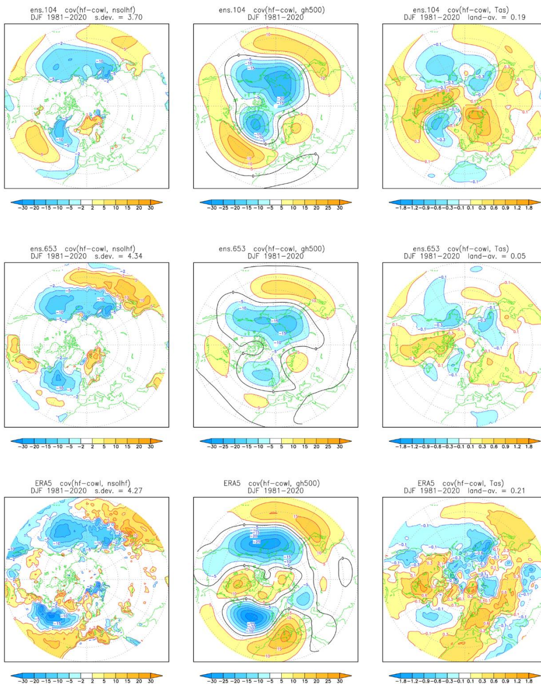
Figure 14: Covariances of downward non-solar heat flux (left, in \text{W/m}^2 ), 500-hPa height (centre, in m) and SAT (right, in ^{\circ}\text{K} ) with the HF-COWL index in DJF 1981-2020, as defined in sect. 4.3. Top row: from coupled ensemble (ens.104). Middle row: from ensemble with prescribed SST (ens.653). Bottom row: from ERA5 data.
