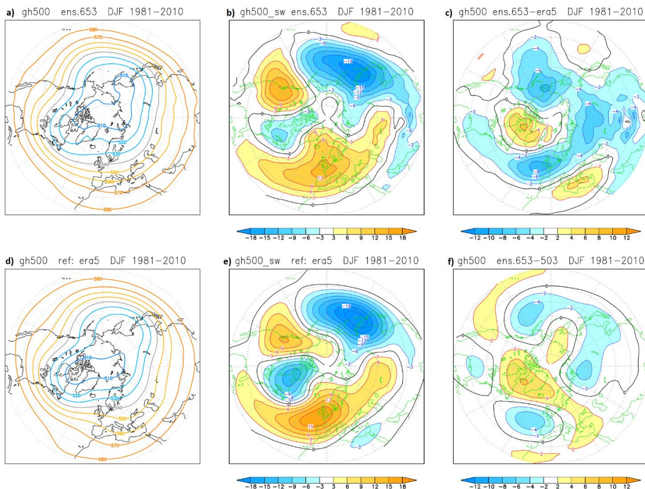
Figure 8: Left column: climatology of 500-hPa geopotential height for DJF 1981-2010 (in dam), from: a) the ensemble with prescribed SST (ens.653), and d) ERA5 data. Middle column ( b, e ): as on left column, but for the stationary waves at 500 hPa (i.e differences from the zonal-mean climatology). c) bias of the 500-hPa height ensemble climatology with respect to ERA5. f) difference with respect to an ensemble with v.42 dynamics but v.41 parametrizations (ens.503).
