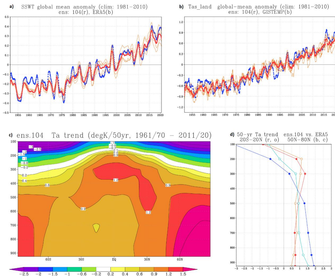
Figure 10: Top row: time series of global and annual-mean variability of a) surface sea-water temperature (SSWT), and b) SAT over land, from the coupled SPEEDY-TOM3 ensemble for 1951-2020 (ens.104). All data are anomalies from a 1981-2010 climatology, in °K. Red curve: ensemble mean; orange curves: individual ensemble members; blue curve: observational data from ERA5 (for SSWT) and GISTEMPv4 (for land SAT). Bottom row: linear trends of atmospheric temperature computed from overlapping 10-yr means, from 1961/70 to 2011/20. Units: °K/(50 yr). c): vertical cross section from the coupled ensemble; d): vertical profiles of trends integrated in two latitudinal bands, from the ensemble in 20S-20N (red curve) and 50N-80N (blue curve), and from ERA5 in 20S-20N (orange curve) and 50N-80N (cyan curve).
