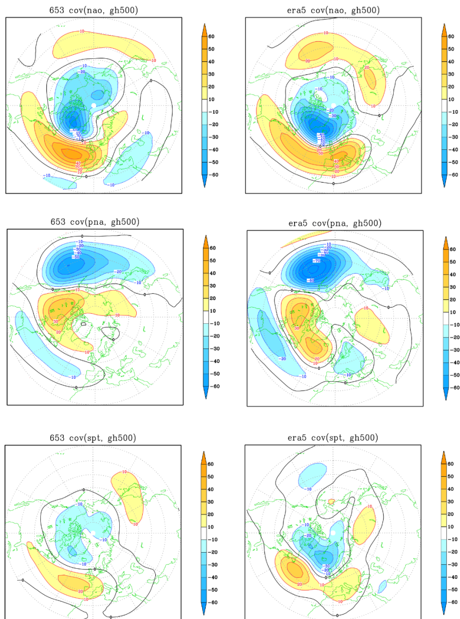
490 Figure 9: Covariance of JF 500-hPa height (in m) with the NAO (top), PNA (centre) and SPT (bottom) indices, for the ensemble with prescribed SST (ens.653, left) and ERA5 data (right) in JF 1981-2020.
