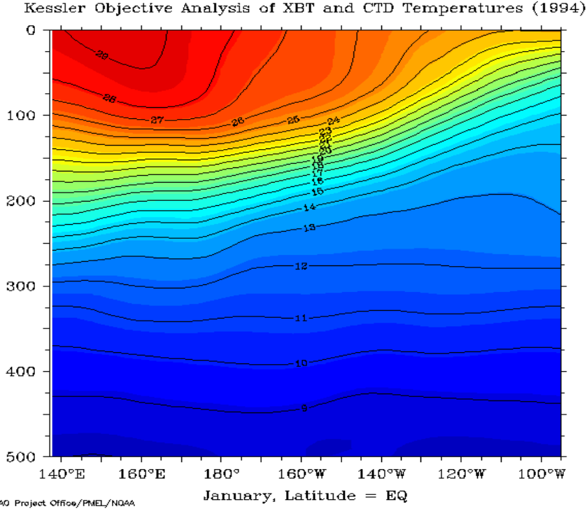
Figure 16: Average January temperature as a function of depths and longitude along the equator. Map from Pacific Marine Environmental Laboratory of NOAA, Seattle.
