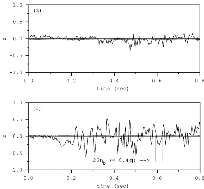
FIG. 8. Sample z traces for Schmidt number ratio of (a) 4 (group I) and (b) 18 (group II). The magnitude of the system noise is indicated. The size of a sample structure is indicated in (b) in terms of the Batchelor scale, \eta_b for basic blue 3 and for the Kolmogorov scale, \eta , of the flow. The two dotted lines in (a) and (b) bracket the total system noise.
