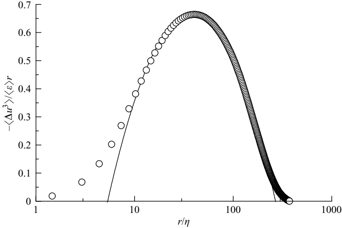
FIGURE 2. Normalized third-order structure function -\Delta u_r^3/\langle \varepsilon \rangle r against \log(r/\eta) . The DNS data are from Gotoh et al. (2002), R_\lambda = 125 . The solid parabola corresponds to (2.12).
