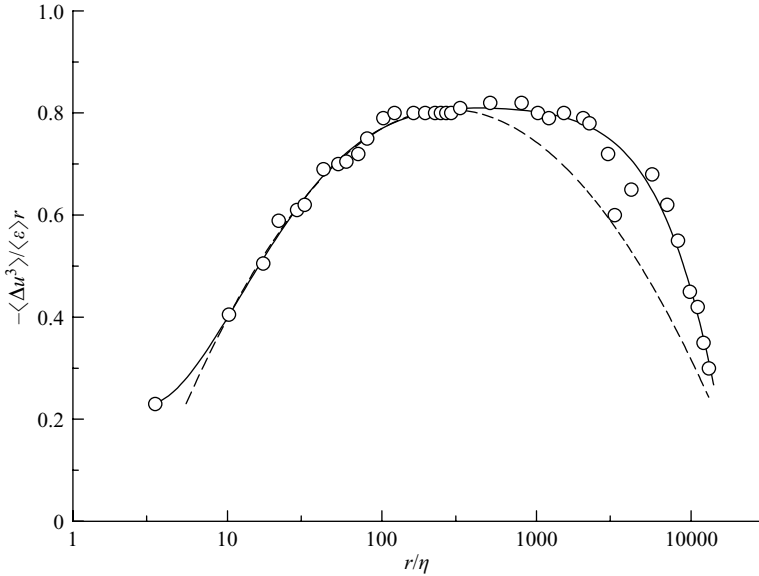
FIGURE 7. As in figure 2 but for an atmospheric experiment (Sreenivasan & Dhruva 1998) at R_\lambda = 10400 . The solid curve corresponds to the expansion (2.9) up to the sixth order. The dashed parabola is (2.12) (i.e. (2.9) with just two terms in the expansion).
