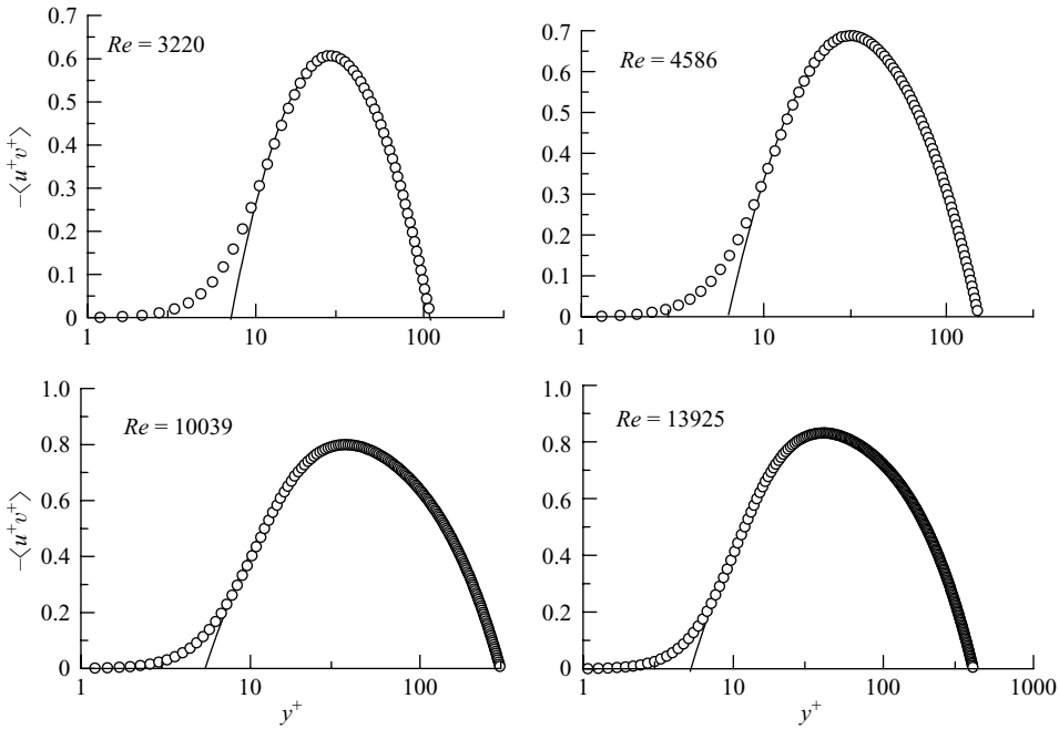
FIGURE 10. Plots of the Reynolds shear stress from the direct numerical simulations of a channel flow (Iwamoto, Suzuki & Kasagi 2002), for four different Reynolds numbers, Re , based on the bulk mean velocity and the width of the channel. The data have been fitted by the two-term expansion (3.3). The fit is very good for y^+ > 10 .
