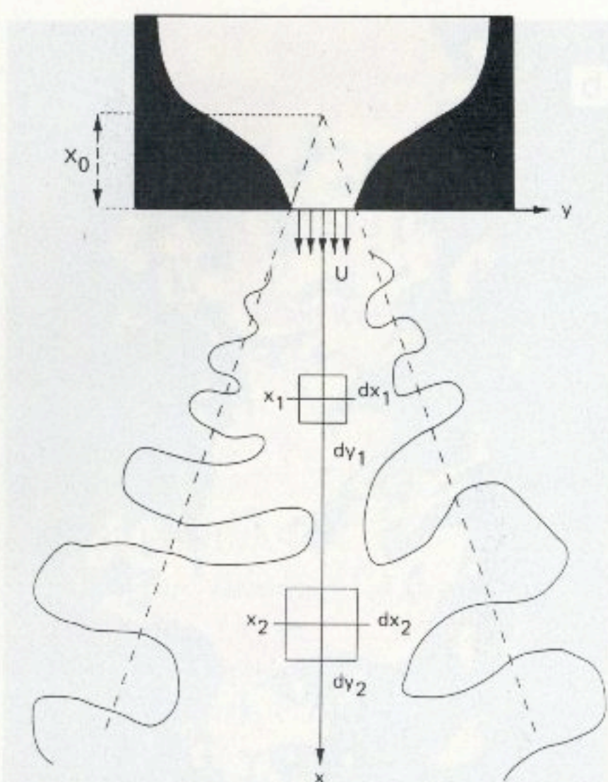
Fig. 2. A schematic of the jet. The linear growth rate of the far field extrapolates to zero at a visual origin x_0 which in this case is about 3\frac{1}{2} nozzle diameters upstream of the nozzle. The nozzle contour and upstream flow management is standard. See ref. [11] for details. The basis of conformal mapping, eq. (7), is that the area element dx_1 dy_1 centered at x_1 grows linearly to the area element dx_2 dy_2 centered at x_2 . The interface convolutions are only schematic emphasizing downstream growth of scales, and should not be interpreted literally.
