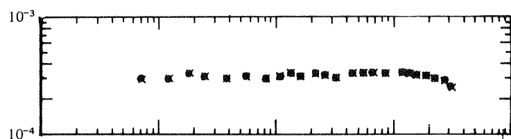
FIGURE 23. Spectral densities of random white noise. ●, total noise signal. ×, 'superposed' fraction of noise.
