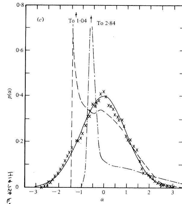
FIGURE 17. Probability density functions. (a) \times , \alpha = u_s/u_s'' ; ---, v_i/v_i' ; - - -, u/u' ; (b) \times , \alpha = v_s/v_s'' ; ---, v_i/v_i' ; - - -, v/v' ; (c) \times , \alpha = \theta_s/\theta_s'' ; ---, \theta_i/\theta_i' ; - - -, \theta/\theta' . For superposed turbulence \bar{T}\bar{U}_a/L = 2.5 , \Delta\bar{T}/\bar{T} = \pm 0.2 . —, Gaussian.
