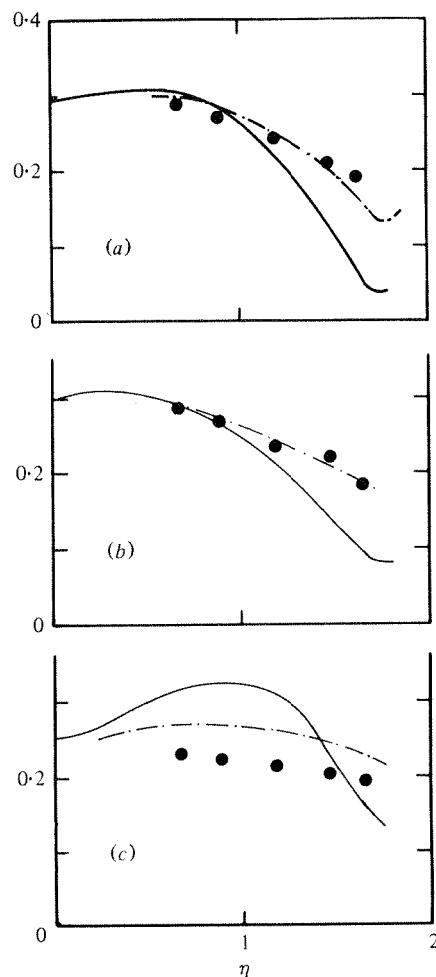
FIGURE 10. R.m.s. velocity and temperature fluctuations across the jet. (a) ●, u''_s/\bar{U}_0 ; —, u'/\bar{U}_0 ; - - -, u'_i/\bar{U}_0 . (b) ●, u''_{sc}/\bar{U}_0 ; —, v'/\bar{U}_0 ; - - -, v'_i/\bar{U}_0 . (c) ●, \theta''_{sc}/\bar{\Theta}_0 ; —, \theta'/\bar{\Theta}_0 ; - - -, \theta'_i/\bar{\Theta}_0 .
