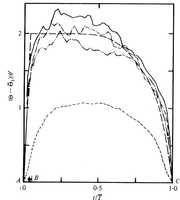
FIGURE 6. Ensemble average distributions of excursions of various durations in the temperature signal, \eta = 0.89 : —, \bar{T}\bar{U}_a/L = 0.38 , \Delta\bar{T}/\bar{T} = \pm 0.5 , N = 194 ; - - -, 1.12 , \pm 0.11 , 84 ; — · —, 1.63 , \pm 0.08 , 66 ; — — —, 2.25 , \pm 0.11 , 112 .
