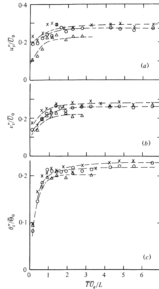
FIGURE 9. Variation of the 'r.m.s.' values of u_s , v_s and \theta_s as a function of \bar{T} . Broken lines are drawn through the points for clarity. \times , \eta = 0.67 ; \circ , 0.89 ; \triangle , 1.48 . (a) u_s''/\bar{U}_0 ; (b) v_s''/\bar{U}_0 ; (c) \theta_s''/\bar{\Theta}_0 .
