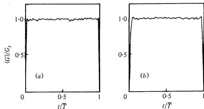
FIGURE 22. Ensemble averages for random white noise. (a) \bar{T} = 150 sampling intervals. (b) \bar{T} = 50 sampling intervals. \Delta\bar{T}/\bar{T} = \pm 0.20 .
