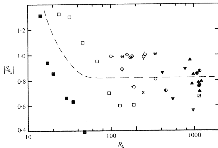
FIGURE 1. Variation of |S_{\theta_x}| with R_\lambda . Gibson et al. (1977): \circ , atmospheric boundary layer; \bullet , heated jet; \blacktriangle , heated wake; \otimes , cooled wake, \blacktriangle , Mestayer et al. (1976), heated boundary layer. \nabla , Gibson et al. (1970), atmospheric boundary layer (corrected for velocity sensitivity); \times , Antonia & Van Atta (1975), heated jet. Freymuth & Uberoi (1971, 1973): \square , heated two-dimensional wake; \blacksquare , heated axisymmetric wake. \ominus , \oplus , \odot , \oslash , Sreenivasan, Antonia & Danh (1977), heated boundary layer. \square , our unpublished data, atmospheric surface layer. \circ , \odot , \oplus , \otimes , present data, axisymmetric heated jet, \eta = 0, 0.89, 1.15, 1.48 and 1.63 respectively. ---, suggested mean trend.
