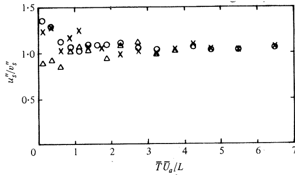
FIGURE 12. Ratio of r.m.s. velocity fluctuations of the superposed turbulence as a function of \bar{T} over which they are defined. \times , \eta = 0.67 ; \circ , \eta = 0.89 ; \triangle , \eta = 1.48 .
