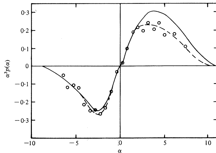
FIGURE 19. The integrand function for the evaluation of skewness of temperature derivatives. \eta = 1.48 . —, \alpha = \theta/\theta' . \circ , \alpha = \theta_s/\theta_s'' . ( \bar{T}\bar{U}_a/L = 2.5 , \Delta\bar{T}/\bar{T} = \pm 0.2 .) ---, suggested mean through the points.
