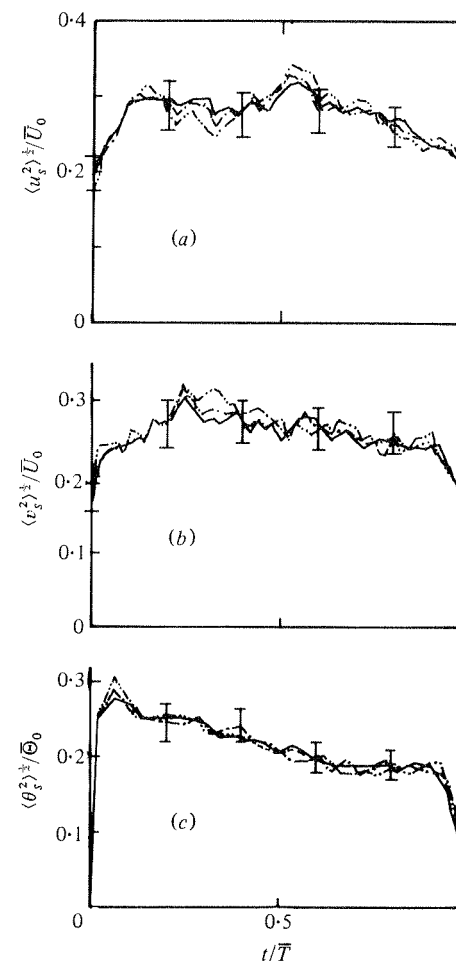
FIGURE 11. R.m.s. velocity and temperature fluctuations about the respective ensemble averages. \eta = 0.89 . —, \Delta\bar{T}/\bar{T} = \pm 0.28 ; - - -, \pm 0.20 ; - · - ·, \pm 0.12 . Vertical bars indicate confidence intervals with 95% confidence level, \Delta\bar{T}/\bar{T} = \pm 0.20 .
