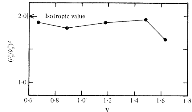
FIGURE 14. Ratio of mean-square derivatives of velocity fluctuations of superposed turbulence.
