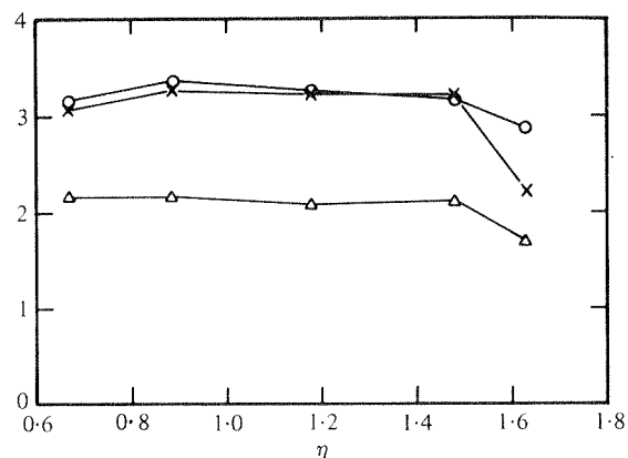
FIGURE 15. Ratio of r.m.s. derivatives of superposed turbulence to those of large scale. ○, u_s''/u_L'' ; ×, v_s''/u_L'' ; Δ, \theta_s''/\theta_L'' .
