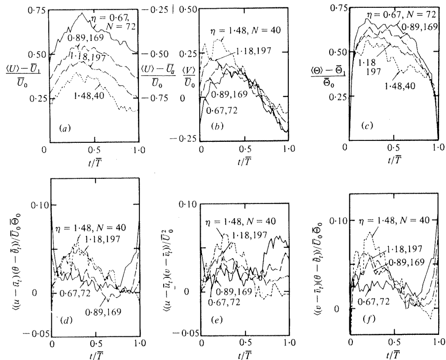
FIGURE 7. Ensemble-averaged distributions of U , V , \Theta and of their products in bulges of duration \bar{T} = 2.5L/\bar{U}_a ; \Delta\bar{T}/\bar{T} = \pm 0.2 . ( N refers to the number of bulges found at the particular value of \eta .)
