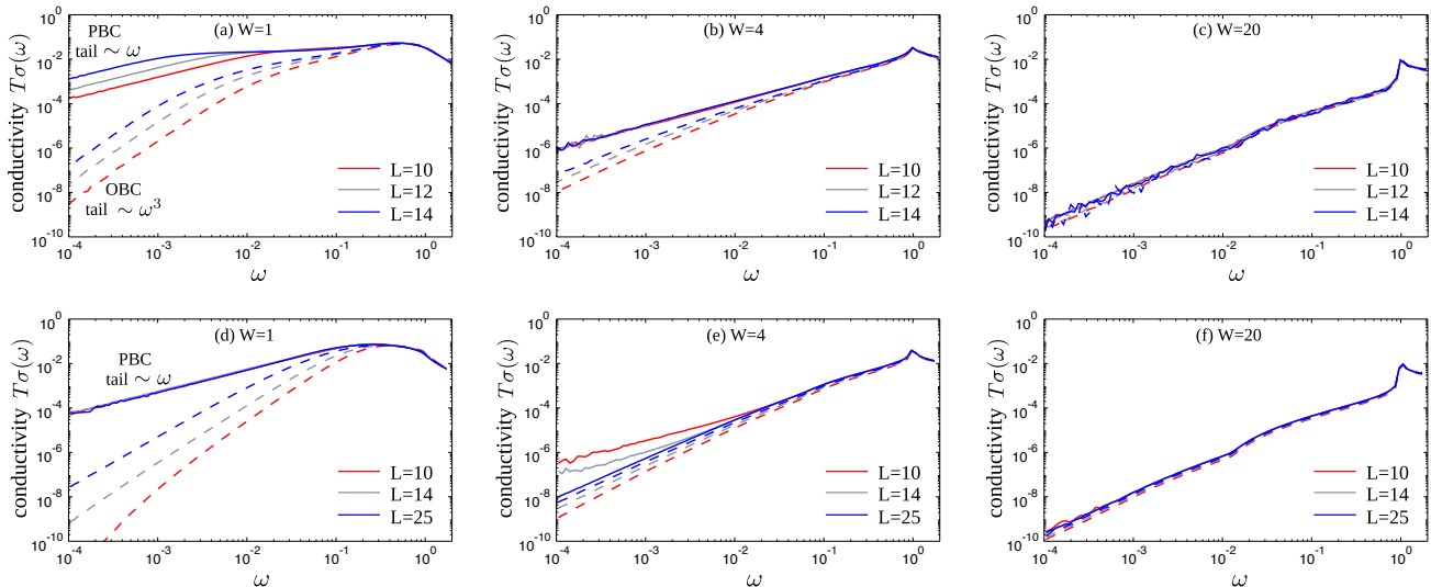
FIG. 4. (Color online) (a)–(c) Frequency dependence of ac conductivity in the interacting system with periodic and open boundary conditions (solid and dashed lines respectively) for three values of disorder W , corresponding to the thermal phase (left), near-critical regime (center), and deeply localized phase (right). The lowest-frequency finite-size behavior in the thermal regime goes as \sigma \sim \omega for periodic boundary conditions and \sigma \sim \omega^3 for open boundary conditions, as discussed in the text. (d)–(f) Frequency dependence of ac conductivity in noninteracting systems, for disorder values corresponding to those in panels (a)–(c). Again, solid lines represent periodic boundary conditions and dashed lines represent open boundary conditions.
