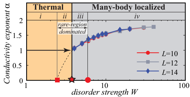
FIG. 1. (Color online) ac conductivity exponent \alpha of a disordered one-dimensional system across the many-body localization transition, showing four regimes: (i) the diffusive thermal phase; (ii) the subdiffusive thermal phase [31], which exists only in one dimension; and (iii, iv) the MBL phase. The MBL phase is divided into an “MBL-Griffiths” regime (iii) in which low-frequency response is dominated by rare critical or thermal regions, and an “MBL-Mott” regime (iv) in which it is dominated by pairs of resonant configurations. Our main predictions are that the exponent \alpha \rightarrow 1 [i.e., \sigma \sim \omega ] as the MBL transition is approached from the localized side, and that 1 \leq \alpha < 2 throughout the MBL phase. These are consistent with numerical simulations of a nearest-neighbor random-field XXZ chain (shown in the plot). In the thermal phase, finite-size effects are strong, and a more careful analysis [31] is needed to extract the conductivity exponent.
