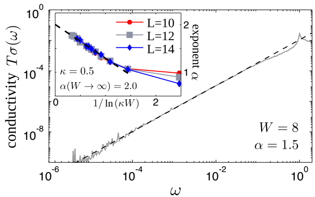
FIG. 3. (Color online) Main panel: conductivity as a function of frequency in the random field XXZ chain for system size L = 14 and disorder bandwidth W = 8 , showing multiple decades of power-law behavior. Inset: behavior of the conductivity exponent deep in the MBL phase is consistent with the many-body Mott prediction (see main text) that 2 - \alpha \sim \zeta , combined with the perturbative estimate \zeta \sim 1/\ln(W/J) .
