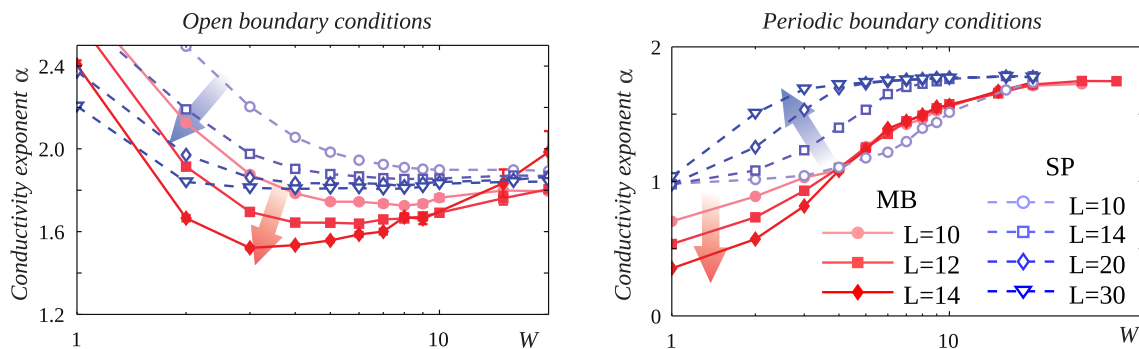
FIG. 5. (Color online) Conductivity exponent for interacting spin chains (solid red lines) and the corresponding noninteracting chains (dashed blue lines) as a function of disorder W , for various system sizes. The left panel shows data for open boundary conditions (OBCs), and the right panel for periodic boundary conditions (PBCs). Exponents are extracted from the frequency regime 10^{-4} \leq \omega \leq 5 \times 10^{-3} (OBC) and 10^{-4} \leq \omega \leq J^2/(4W) (PBC). Arrows indicate the evolution of the exponent with increasing system size. For OBCs, the exponent crosses over from the finite-size value \alpha = 3 to the Mott value \alpha \simeq 2 with increasing disorder. The crossover is nonmonotonic for interacting systems but monotonic for noninteracting systems, as discussed in the text. For PBCs, noninteracting systems again exhibit a monotonic crossover from the finite-size exponent \alpha = 1 to the Mott exponent \alpha = 2 . However, the exponent for interacting systems drops well below the finite-size value \alpha = 1 , in the regime where these systems are thermal. Moreover, finite-size effects on \alpha seem negligible throughout the MBL phase.
