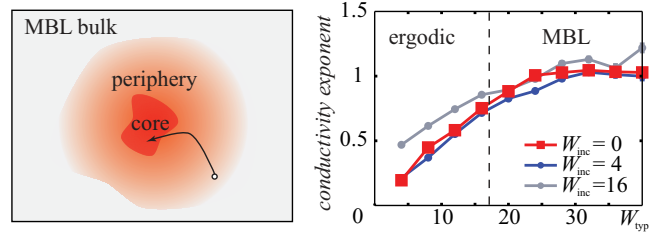
FIG. 2. (Color online) Left: schematic of the structure of a thermal inclusion in the MBL phase, showing its core (the microscopically rare thermal region), the periphery (the typical surroundings that get strongly entangled with the rare region), and the typical MBL surroundings where the core does not flip the local effective spins. Low-frequency transport occurs through transport between the periphery and the core. Right: numerically computed conductivity exponent \alpha of an XXZ chain of size L = 12 with integrability-breaking next-to-nearest-neighbor exchange coupling that contains a thermal or critical inclusion (i.e., a region that is locally thermal or critical) of four sites. W_{typ} is the typical value of disorder, and three different disorder values for the inclusion W_{inc} are shown. When the typical system is in the MBL phase ( W_{typ} > 8 ), the conductivity exponent saturates to near 1, consistent with the discussion in the main text.
