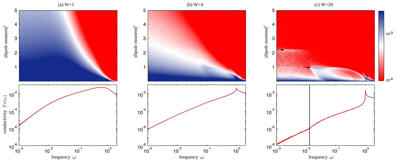
FIG. 6. (Color online) Distribution of squares of dipole moment matrix elements (i.e., |\langle n | \sum_j j S_j^z | m \rangle|^2 ) contributing to the conductivity at each frequency, for disorder corresponding to thermal phase (left), critical region (center), and MBL phase (right), all with open boundary conditions. In (c) the arrows mark the peaks corresponding to two-site and three-site hops in the MBL phase (see text); we expect the n -site peak to vanish at a frequency \sim 1/W^{n-1} , giving rise to a “shoulder” in the conductivity. Lower panel: frequency dependence of the conductivity. Note that the different regimes of behavior in \sigma(\omega) can be matched with features in the dipole moment distribution.
