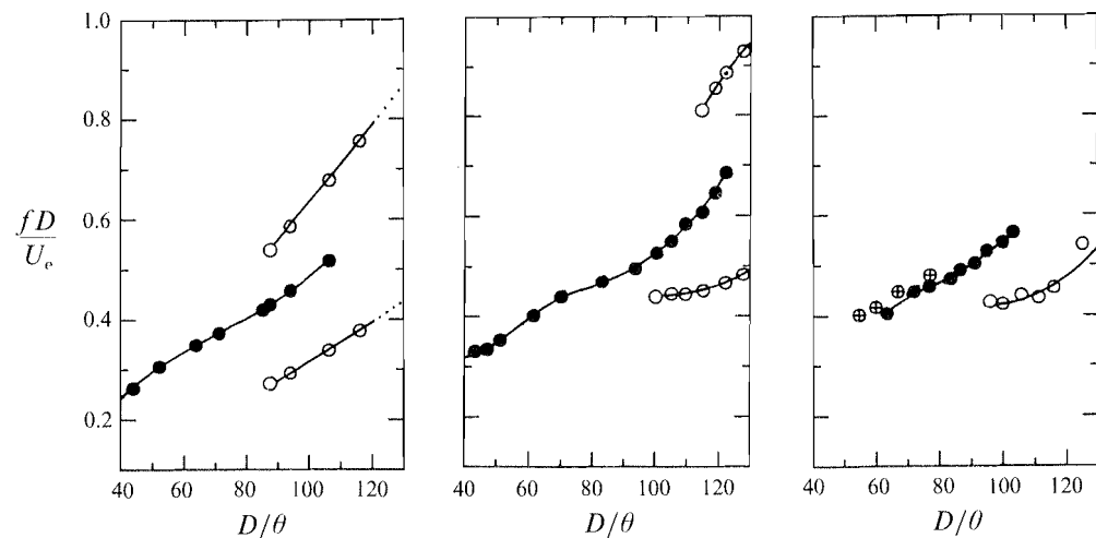
FIGURE 16. Non-dimensional frequency fD/U_e as a function of D/\theta for various values of S : x/D = 0.10 ; from left to right S = 0.14 , 0.29 and 0.48 respectively. \bullet , oscillating mode from present experiments; \circ , additional prominent disturbance modes in present facility; \oplus , oscillating mode (Mode II) in the heated air jet (Monkewitz et al. 1990).
