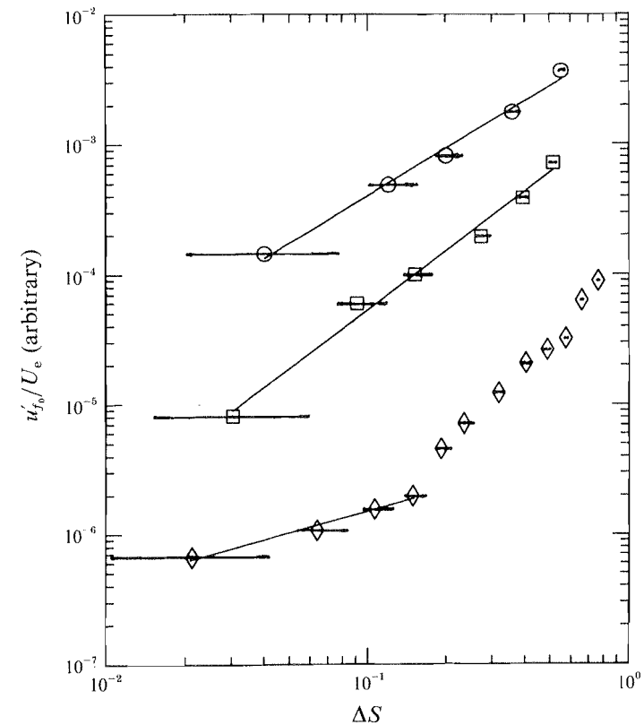
FIGURE 20. Square root of the power spectral density of u' at f_0 , u'_{f_0} , normalized by U_e , and plotted as a function of \Delta S = (S_0 - S)/S_0 for various D/\theta : The power spectrum was measured with respect to an arbitrary reference voltage which was constant for all of the measurements. \diamond , D/\theta = 83 ; \square , D/\theta = 62.5 ; \circ , D/\theta = 50 . S = 0.14 ; r/D = 0.55 . The uncertainty in S_0 (see figure 19) is the primary source of uncertainty in \Delta S .
