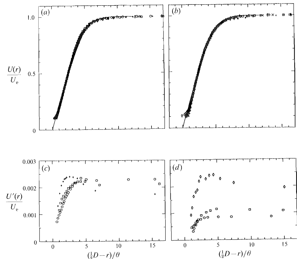
FIGURE 4. Variation of streamwise velocity in the nozzle plane ( x = 0.06 \text{ mm} ) at various Reynolds numbers: \circ , Re = 16000 ; \square , Re = 7000 ; \times , Re = 5000 ; * , Re = 3500 ; + , Re = 2700 ; \diamond , Re = 2100 . (a) U(r)/U_e for ASME nozzle. D = 13.3 \text{ mm} ; (b) U(r)/U_e for cubic equation nozzle, D = 9.3 \text{ mm} . (c) Fluctuation amplitude u'/U_e for ASME nozzle; D = 13.3 \text{ mm} . (d) Fluctuation amplitude u'/U_e for cubic equation nozzle; D = 9.3 \text{ mm} . Measurements are obtained using a standard hot wire in air jets.
