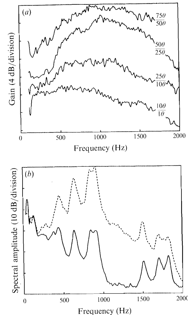
FIGURE 24. (a) Mode amplification as a function of frequency: S = 0.50 ; D/\theta = 83 . Curves are labelled with the appropriate streamwise interval. The gain at each S is determined to within an arbitrary constant factor. (b) Power spectra of u' obtained in the shear layer: —, x/\theta = 1 ; ----, x/\theta = 75 . S = 0.50 ; D/\theta = 83 . The arbitrary reference for the dB scale differs between the two curves.
