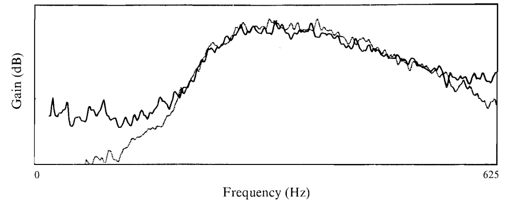
FIGURE 31. Mode amplification between x/\theta = 25 and x/\theta = 75 as a function of frequency for two different radial locations: S = 0.60 ; D/\theta = 62.5 ; ----, potential core; —, r = \frac{1}{2}D + 5\theta . The gain at each r is determined to within an arbitrary constant factor.
