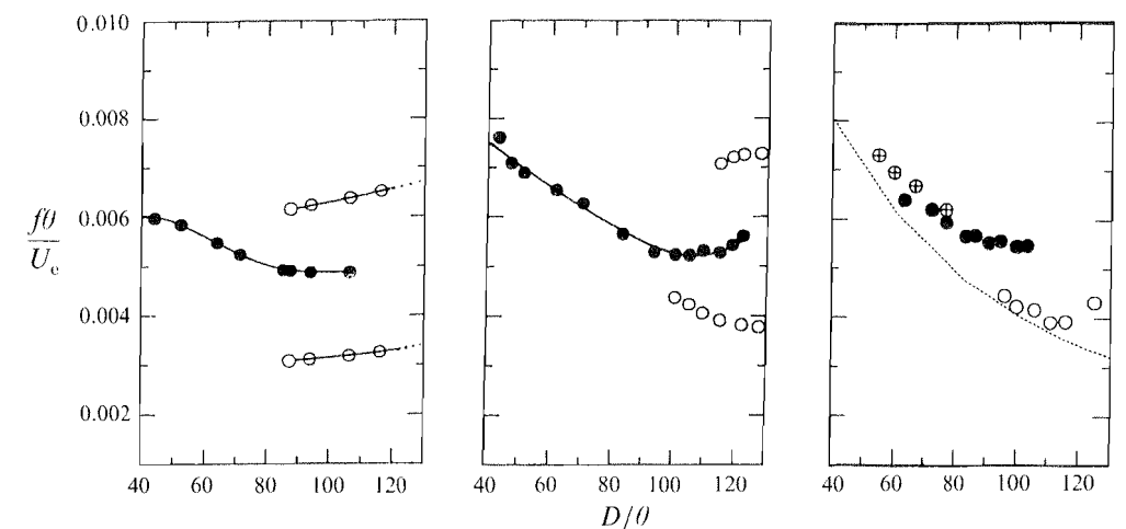
FIGURE 17. Non-dimensional frequency f\theta/U_e as a function of D/\theta : x/D = 0.10 ; \bullet , oscillating mode from present experiments; from left to right S = 0.14 , 0.29 and 0.48 respectively. \circ , additional prominent modes in present facility; \oplus , oscillating mode in the heated air jet (Monkewitz et al. 1990); -----, theory (Monkewitz & Sohn 1988).
