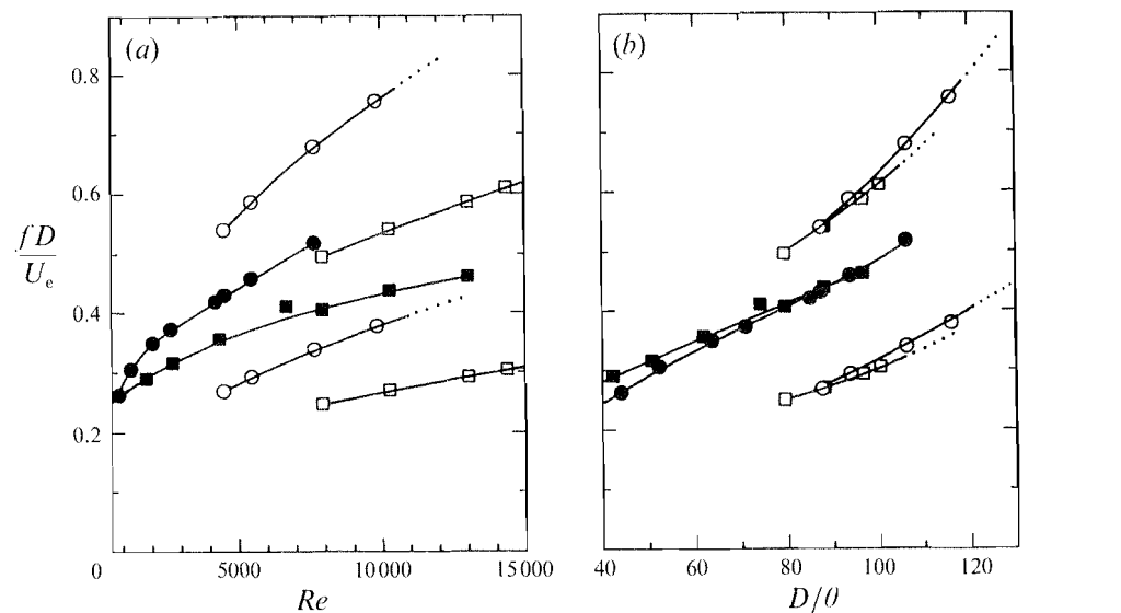
FIGURE 15. Non-dimensional frequency fD/U_e plotted separately as a function of D/\theta and as a function of Re : \circ , D = 9.3 mm; \square , D = 13.3 mm. S = 0.14 ; x/D = 0.10 . Solid symbols represent the oscillating mode; open symbols represent the other broadband modes prevalent in the near-field measurements (see figure 14).
