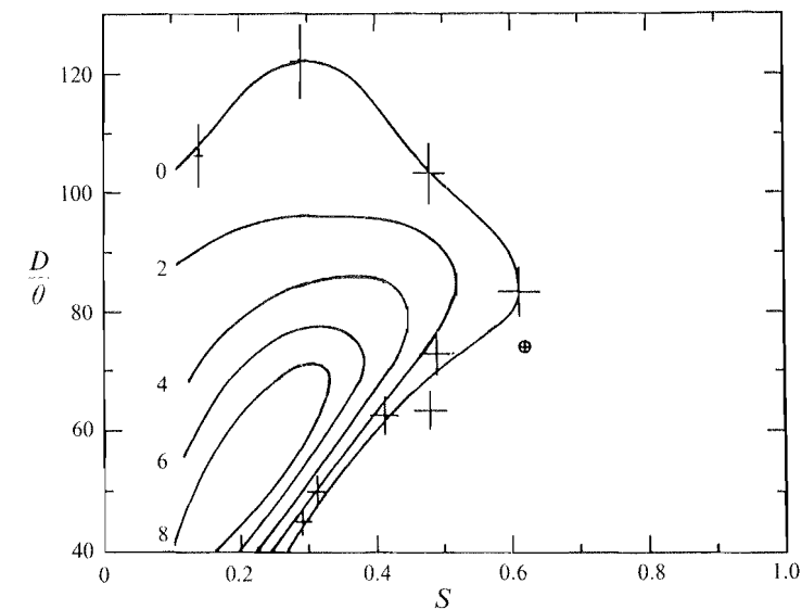
FIGURE 19. Near-field base-to-peak intensity as a function of D/\theta and S : contours are labelled with base-to-peak intensity values. The inner contours correspond to larger and larger peak intensities. Error bars denote uncertainty in experimental determination of onset. \oplus , onset in heated air jets (Monkewitz et al. 1990).
