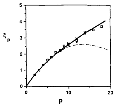
Figure 18 The scaling exponent of the velocity structure function in the inertial range. Symbols correspond to the measurements of Anselmet et al (1984), whereas the continuous curve is obtained from ensemble-averaged D_q results using (6.1) (from Meneveau & Sreenivasan 1987a). The dashed curve is for the log-normal distribution with \mu = 0.26 .
