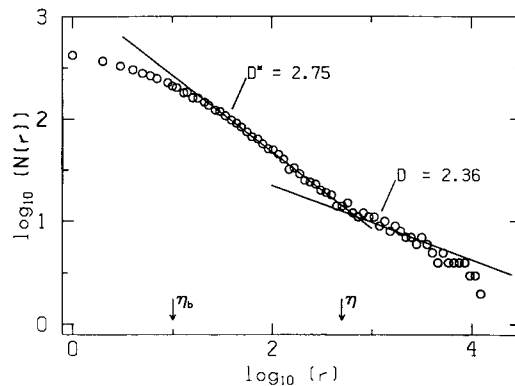
Figure 9 A typical log-log plot of the number N(r) of line elements of size r containing the interface versus the box size r in the B -range. Measurements were made off-axis in the plane wake of a circular cylinder, 75 diameters downstream. The data are generated from single-point fluorescence measurements of the dye concentration, with a spatial resolution comparable to the Batchelor scale and ultrafast temporal response. The negative slopes of the straight parts yield, in the respective scaling regimes, the dimensions of line intersections with the interface. The interface dimension, corresponding to the lines drawn, is 2.36 in the K -range and 2.75 in the B -range. The substantial scatter in the K -range results from the fact that extremely fine resolution of the measurements necessitated the use of a signal length that could not capture many large scales. From Sreenivasan & Prasad (1989).
