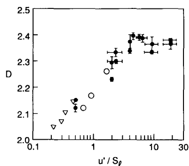
Figure 13 The variation of the fractal dimension in premixed flames as a function of the turbulence level (normalized by the laminar flame speed S_L ). The initial increase appears exponential to a good approximation, and the asymptotic value is comparable to that for scalar interfaces in isothermal flows. Filled circles are from Mantzaras et al (1989a,b), triangles from North & Santaviceca (1990), and open circles from Murayama & Takeno (1988).
