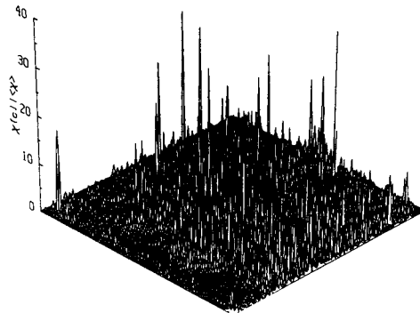
Figure 14b The quantity \chi is plotted for a small rectangular area in a planar section of a jet. All three components of \chi have been measured here; the third component has been estimated by differencing concentration levels between two parallel planes separated by about 4\eta . This figure illustrates quantitatively the spatial intermittency of the dissipation field (from Prasad & Sreenivasan 1990a).
