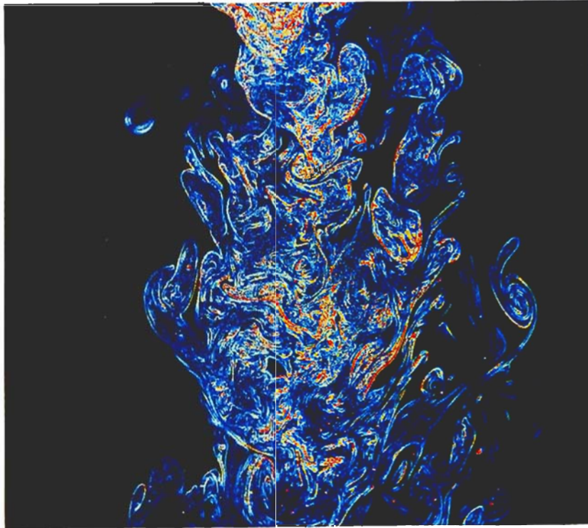
Figure 14a From the LIF map of the concentration field, one can calculate the “dissipation” rate of the variance of concentration fluctuation. This is shown for one realization of a jet at a Reynolds number of 4000. The gradients of the concentration required for computing \chi were approximated by finite differences of the concentration field. Only two components of \chi are included here. The spatial resolution of measurements is estimated to be between \langle \eta \rangle and 2 \langle \eta \rangle . Different colors represent, in some nonlinear scaling, different magnitudes of the dissipation rate; magnitudes increase from deep blue through red. The figure shows that different magnitudes of dissipation inhabit different but intertwined sets. The purpose of the multifractal analysis is to disentangle information about the dimensions of these sets and the strengths of the measures living on them.
