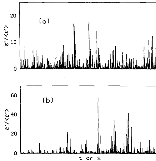
Figure 15 Two typical signals \epsilon' = (du/dt)^2 , serving as the surrogate of the energy dissipation rate, are plotted here upon normalizing by their mean values. Graph (a) was obtained in a standard flat-plate laboratory boundary layer at a momentum-thickness Reynolds number of 3600. The measurement station was 0.2\delta , where \delta is the boundary-layer thickness ( =4 cm). The microscale Reynolds number there was 110. Graph (b) was obtained in the atmospheric surface layer at a height of about 18 m above the ground. The mean wind speed was about 6 \text{ m s}^{-1} , and the estimated microscale Reynolds number was 1800. The increased intermittency at the higher Reynolds number is obvious. This intermittency, representing the fact that there is a definite limit to small-scale mixing, is believed to be an important feature of turbulence (from Meneveau & Sreenivasan 1990b).
