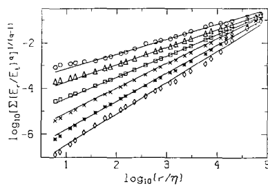
Figure 16 Typical log-log plots of (\Sigma E_r)^{1/(q-1)} versus r for the dissipation field measured in the surface layer of the atmosphere for the conditions as in Figure 15b. E_r in the ordinate is normalized by the total measure E_t in the signal, and the box size is normalized by the estimated Kolmogorov scale \eta . Linear regions in these plots give the generalized dimensions. From top to bottom: q = 4, 2, 0.6, -0.6, -2, and -4 (from Meneveau & Sreenivasan 1990b).
