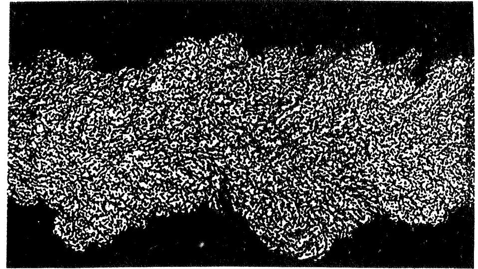
FIGURE 1. A short duration shadowgraph of the wake of a projectile shot through the atmosphere at supersonic speed. This classic photograph made at the Ballistic Research Laboratories, Aberdeen Proving Ground, first appeared in Corrsin & Kistler (1954), and has since been reproduced many times. The remarkably sharp boundary between the turbulent region in the wake and the outside air has led to the notion of a contiguous interface whose properties were explored by Corrsin & Kistler, and several others later.
