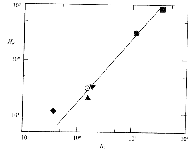
FIGURE 18. The hyperflatness of (dT/dt) . \blacklozenge , Yeh (1971); \bullet , Sreenivasan, Antonia & Danh (unpublished), boundary layer; \blacktriangledown , Antonia & Van Atta (1978), jet; \blacktriangle , Antonia & Van Atta (1978), laboratory boundary layer; \circ , Antonia & Van Atta (1978), atmospheric boundary layer over land; \blacksquare , Park (1976), atmospheric boundary layer over water.
