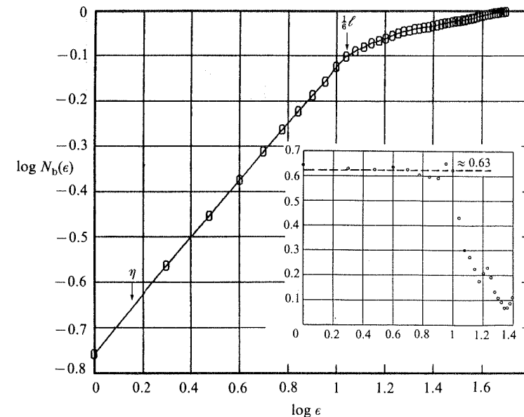
FIGURE 6. The logarithm (to base 10) of the number of boundary points N_b (see figure 5) as a function of the distance \epsilon from the boundary. The flow is a heavily tripped boundary layer, thickness about 10 cm, U_\infty = 2.5 m s ^{-1} . The Kolmogorov and the integral scales are shown for reference. The inset showing the slope gives D_2 = 2 - \text{mean slope} = 1.37 ; D_3 is thus expected to be 2.37.
