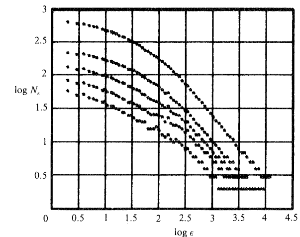
FIGURE 14. The effect of increasing the data segment length used for computing the dimension. The data segment length is, from bottom to top: 50\ell , 83\ell , 132\ell , 200\ell and 430\ell , where \ell is the transverse integral lengthscale. For small lengths, there is a distinct constant-slope region over the scales of interest; this becomes less conspicuous as the signal length increases. For large data segments, one can find a constant-slope region in the scale region far larger than the integral scale; the dimension D_1 is very nearly 1, however.
