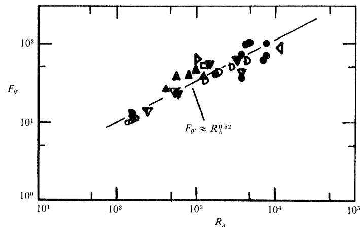
FIGURE 17. The kurtosis of the temperature derivative (dT/dt) . \bullet , McConnell (1976), atmosphere; \triangleleft , Antonia et al. (1980), atmosphere; \mathbb{D} , Antonia & Danh (1977), atmosphere; \circ , Sreenivasan, Antonia & Danh (1977), boundary layer; \blacktriangle , Gibson et al. (1970), atmosphere; \triangleright , Park (1976), atmosphere; \square , McConnell (1976); jet; \nabla , Antonia & Van Atta (1975); \blacklozenge , Antonia & Danh (1977), jet; \blacktriangledown , Gibson & Masiello (1972), jet; \blacktriangledown , Gibson et al. (1970), jet.
